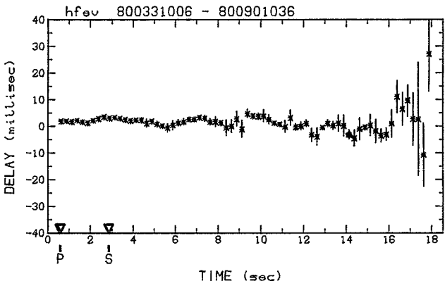
DOUBLET A657 (suite)
