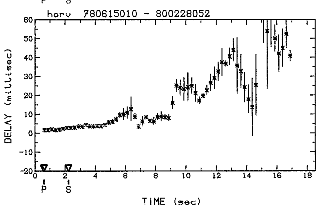
DOUBLET C2 (suite)
