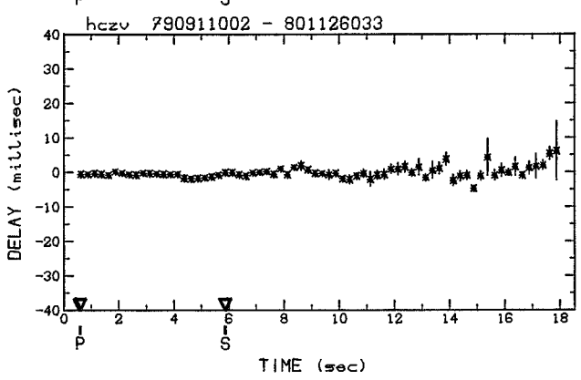
DOUBLET A721 (suite)
