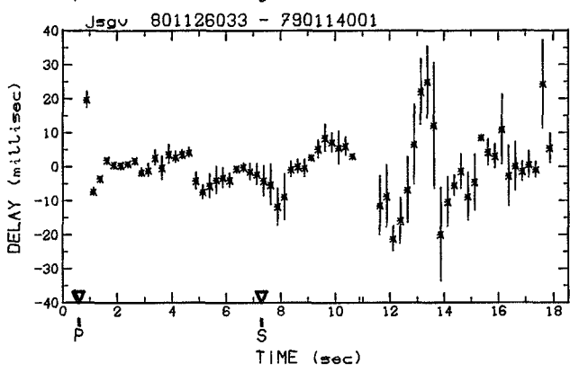
DOUBLET A713 (suite)
