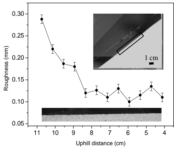
FIG. 11: Spontaneous segregation. The graph indicates the decrease in the roughness amplitude of the pile as we move uphill, suggesting segregation of bigger particles near the lower edge of the heap. The roughness amplitude has been measured as the root mean square of the elevation across 12mm long running windows on the free surface seen in the 7cm-long picture of the lower inset, corresponding to the boxed region indicated in the upper inset. We define the uphill distance as the distance from a point on the surface to the top of the pile.
