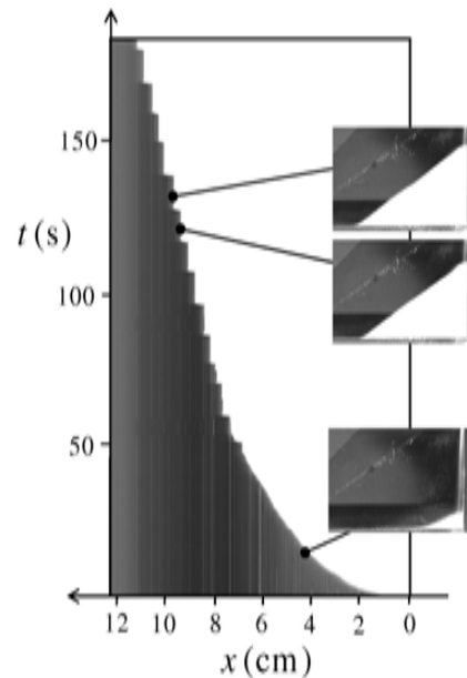
FIG. 9: Spatio-temporal diagram of the growing heap. The diagram was made for a sequence of images taken at every 0.1s to a heap growing in a Hele-Shaw cell with w = 4 mm and F = 0.125 \text{ cm}^3/\text{s} . The cuts were taken along an approximately 12 cm-long horizontal line near the bottom of the cell. As the time goes by, the heap grows continuously, corresponding to a smooth increase of the white area in the diagram. At a critical distance of 7 cm, avalanches start, and the diagram shows a step-like behavior. The insets on the right contains real pictures of the heap illustrating different moments of the spatio-temporal diagram.
