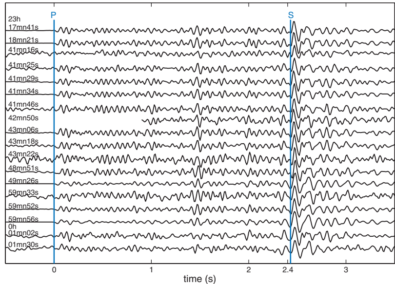
Fig. 2. Records of the foreshocks, arranged in chronological order from top to bottom. The starting time of each trace, the P -wave arrival, and the S -wave are indicated. Each trace is normalized to its peak amplitude, given in table S1. The origin of the time axis corresponds to the P -wave arrival.
